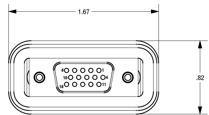
DB15 Female SCALE 1.500
